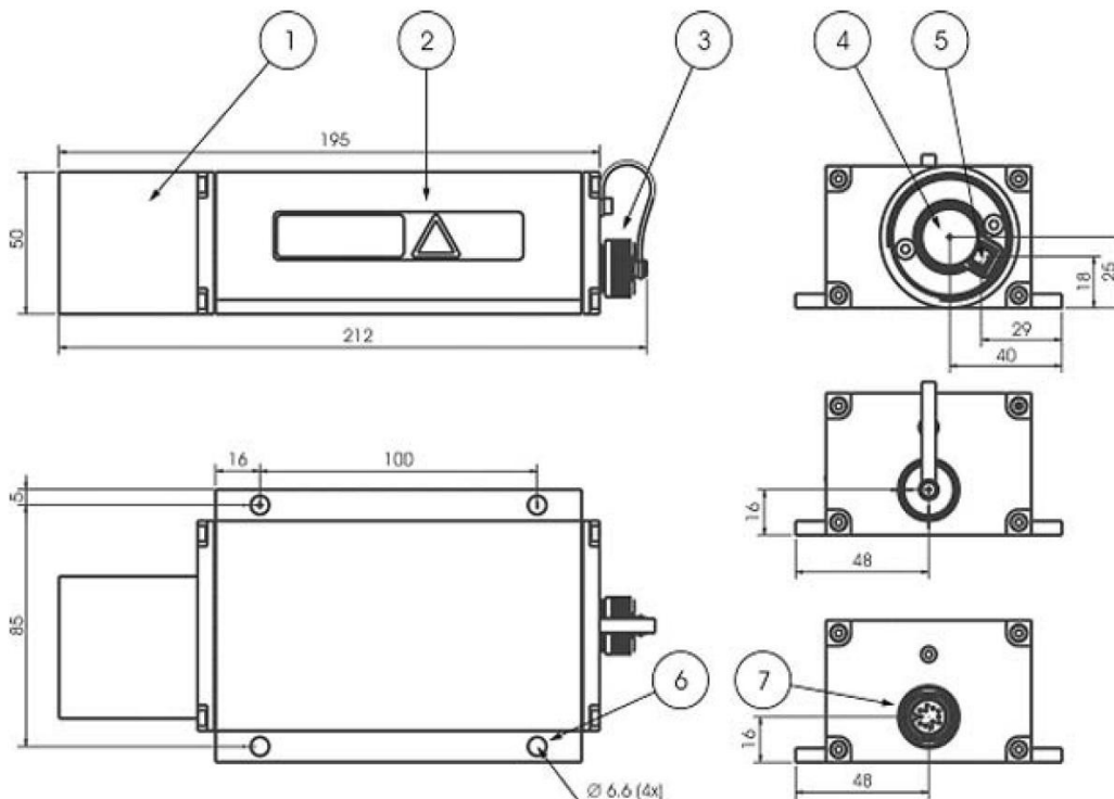
Figure 1: Dimensional drawing
