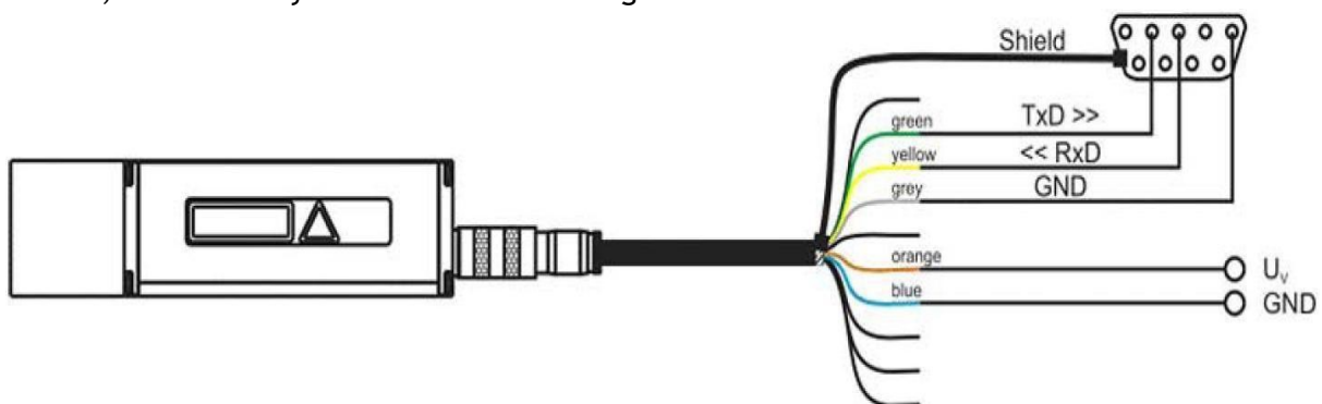
Figure 14: Diagram of RS232 wiring at 9-position D-Sub cable jack
