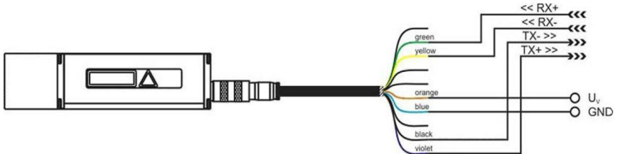
Figure 16: RS422 wiring diagram
